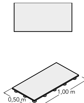
Plaque de base PL 10
